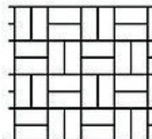
BASKET WEAWE BRICK SIZE: 3 1/2" X 7 1/2" ROLL WIDTH: 33 1/2" JOINT WIDTH: 1/2"
