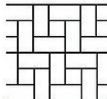
FLANDERS WEAWE FULL BRICK SIZE: 4 1/2" X 10 1/2" ROLL WIDTH: 33" JOINT WIDTH: 1/2"
